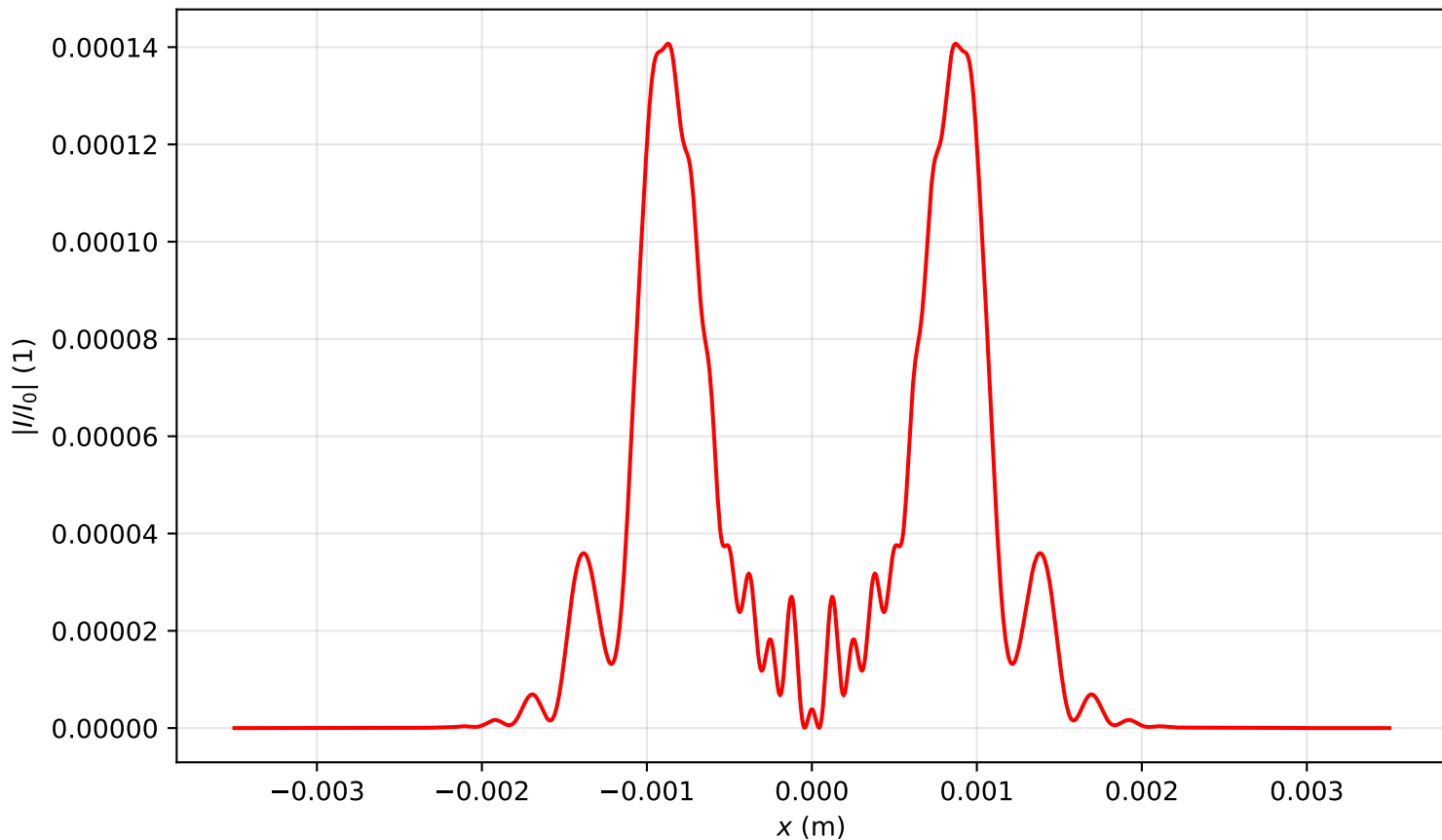
Intensity profile I(x, y = 0, z = 0.716)/I_0 , P_{in}=9.0P_{cr} , artificial time
